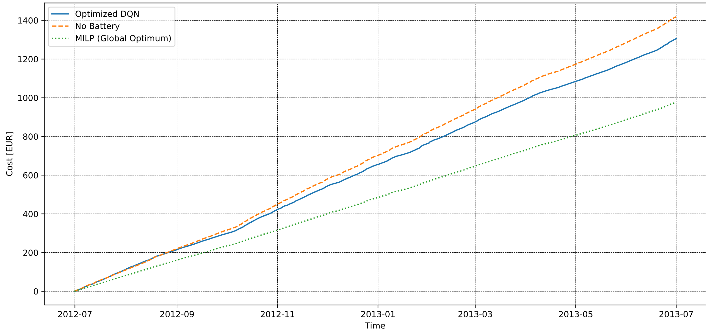
User 290 - Basic Training - Electricity Cost [DQN vs MILP]
